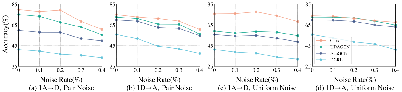
Figure 3: Accuracy on 1A→D and 1D→A with Pair Noise and Uniform Noise on various levels of label noise setting.
