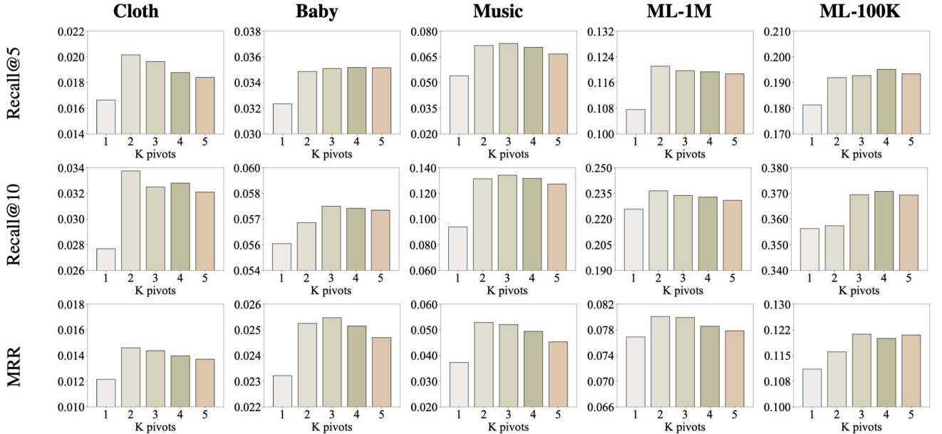
Fig. 4. Performance comparison w.r.t. different settings of the number of pivot timestamps K .
